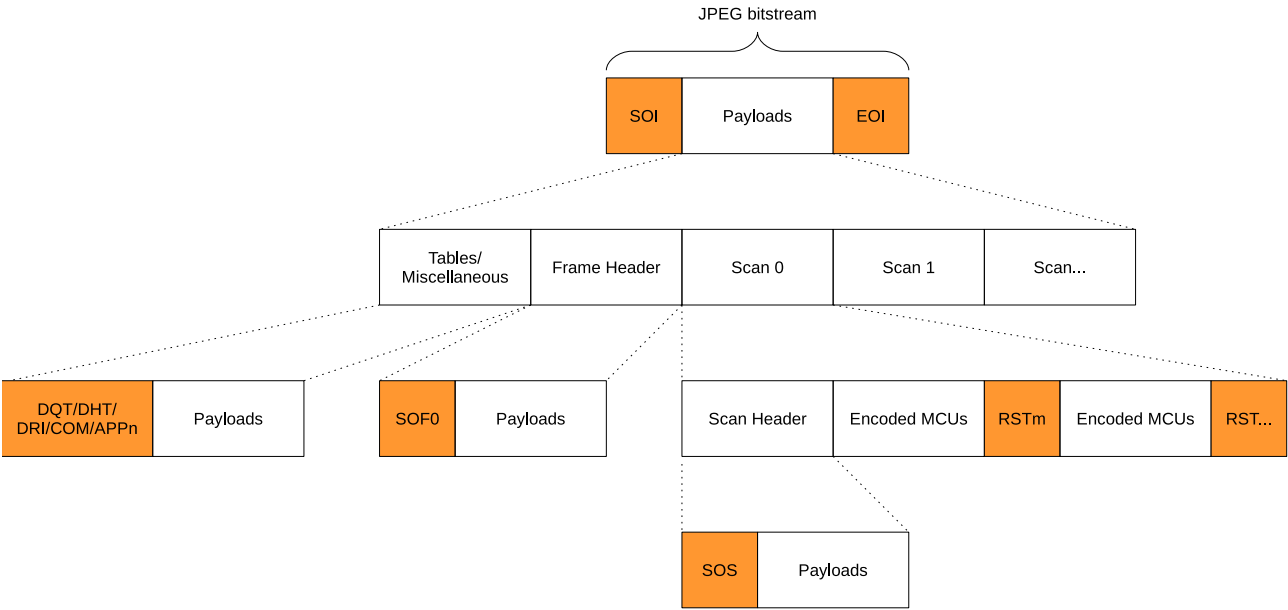
Figure 35.1-1. JPEG Bitstream Format
