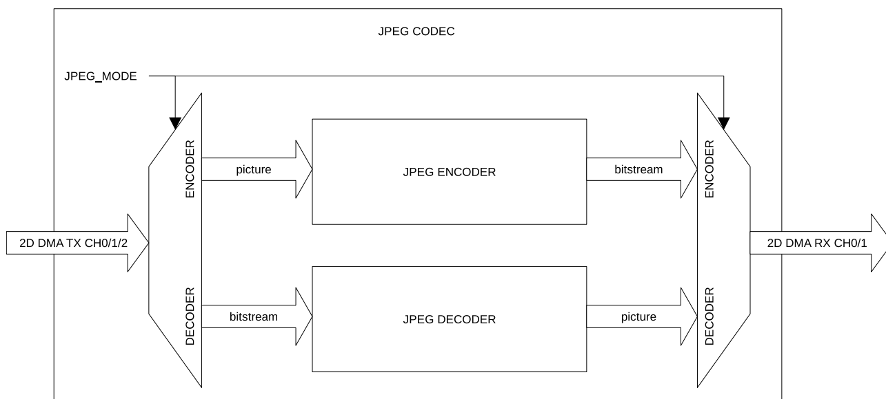
Figure 35.2-1. JPEG codec system connection block diagram
