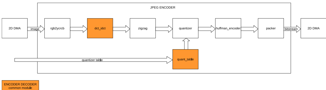
Figure 35.4-1. JPEG encoder architecture
